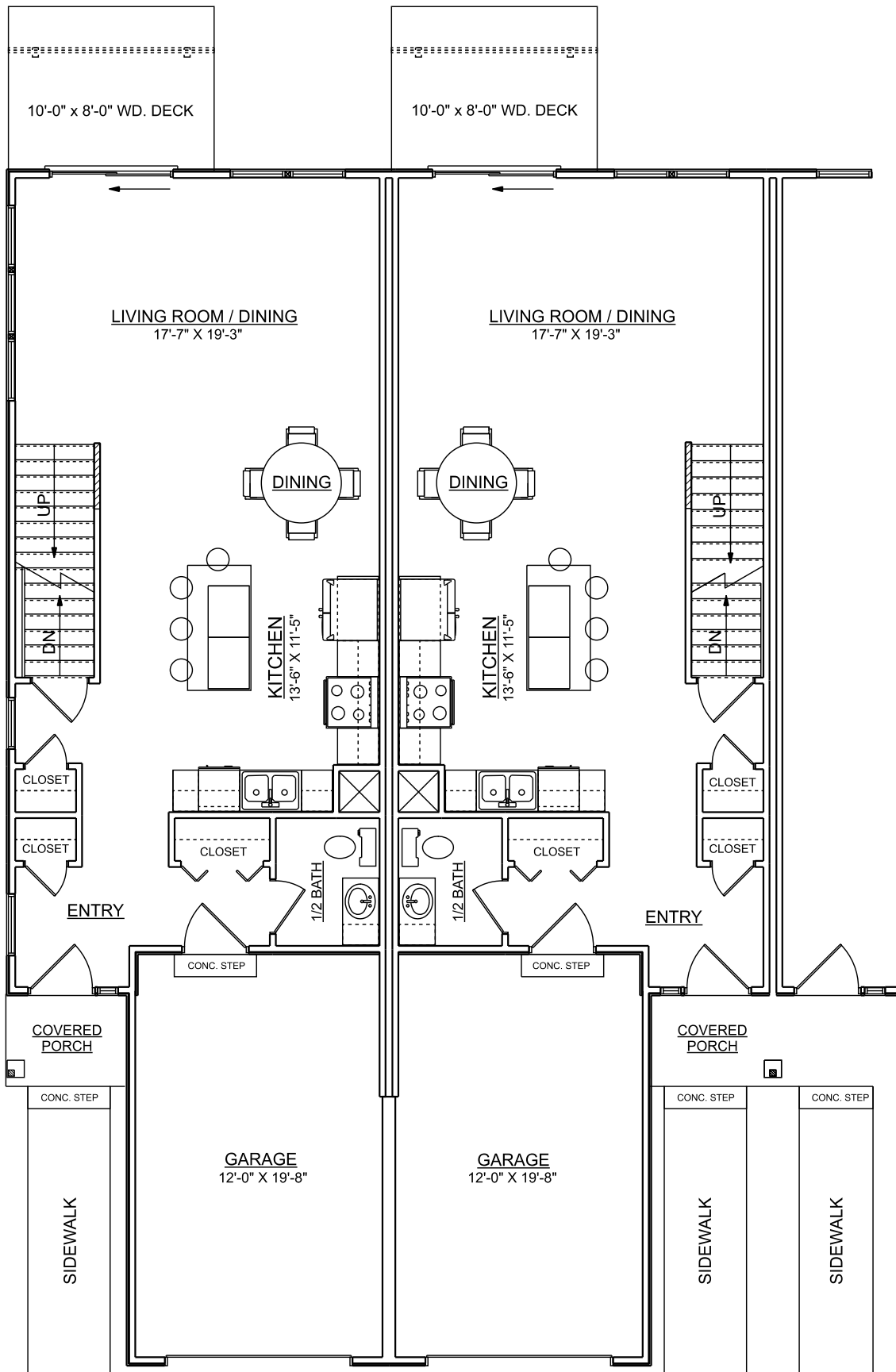
END UNITS MAIN FLOOR PLAN
